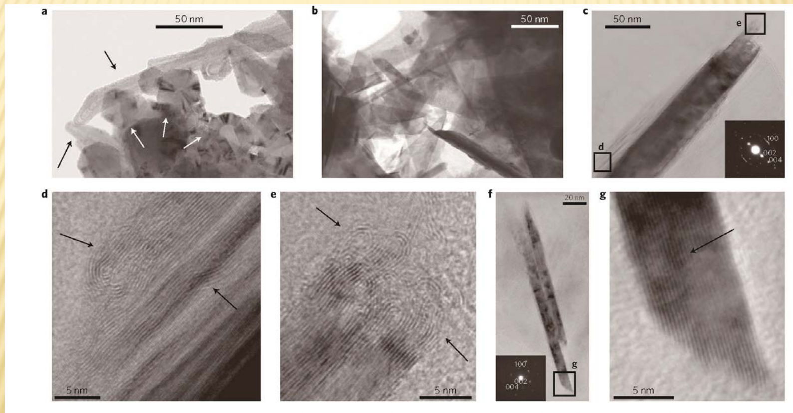
Figure 4 | Transmission electron microscopy images of graphite. a, STEM image of graphite in metasediment (sample 6072906), showing dominance of polygonal and tube-like grains. b, STEM image of secondary graphite (sample 4062002y), showing dominance of sheeted flake grains. c, HRTEM image of graphite in metasediment (sample 6072905). SAED was obtained from area in c . d,e, Magnification of the area marked d and e in c . f,g, HRTEM image of sample 4062002y. SAED was obtained from area in f . g, Magnification of the area marked g in f . Arrows are explained in the main text.
